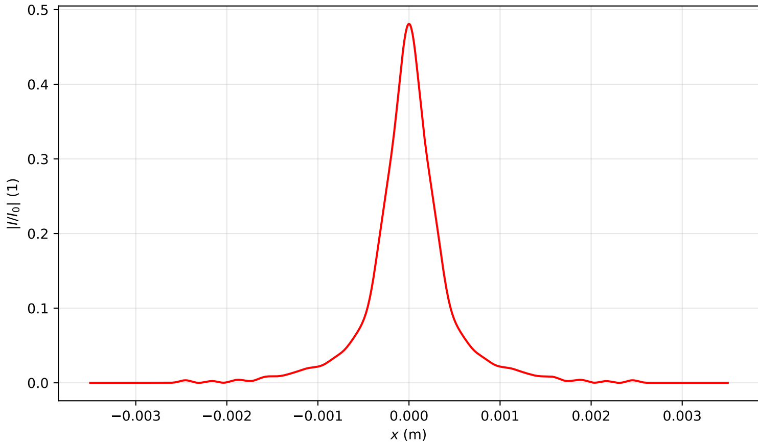
Intensity profile I(x, y = 0, z = 2.229)/I_0 , P_{in}=3.0P_{cr} , artificial time
